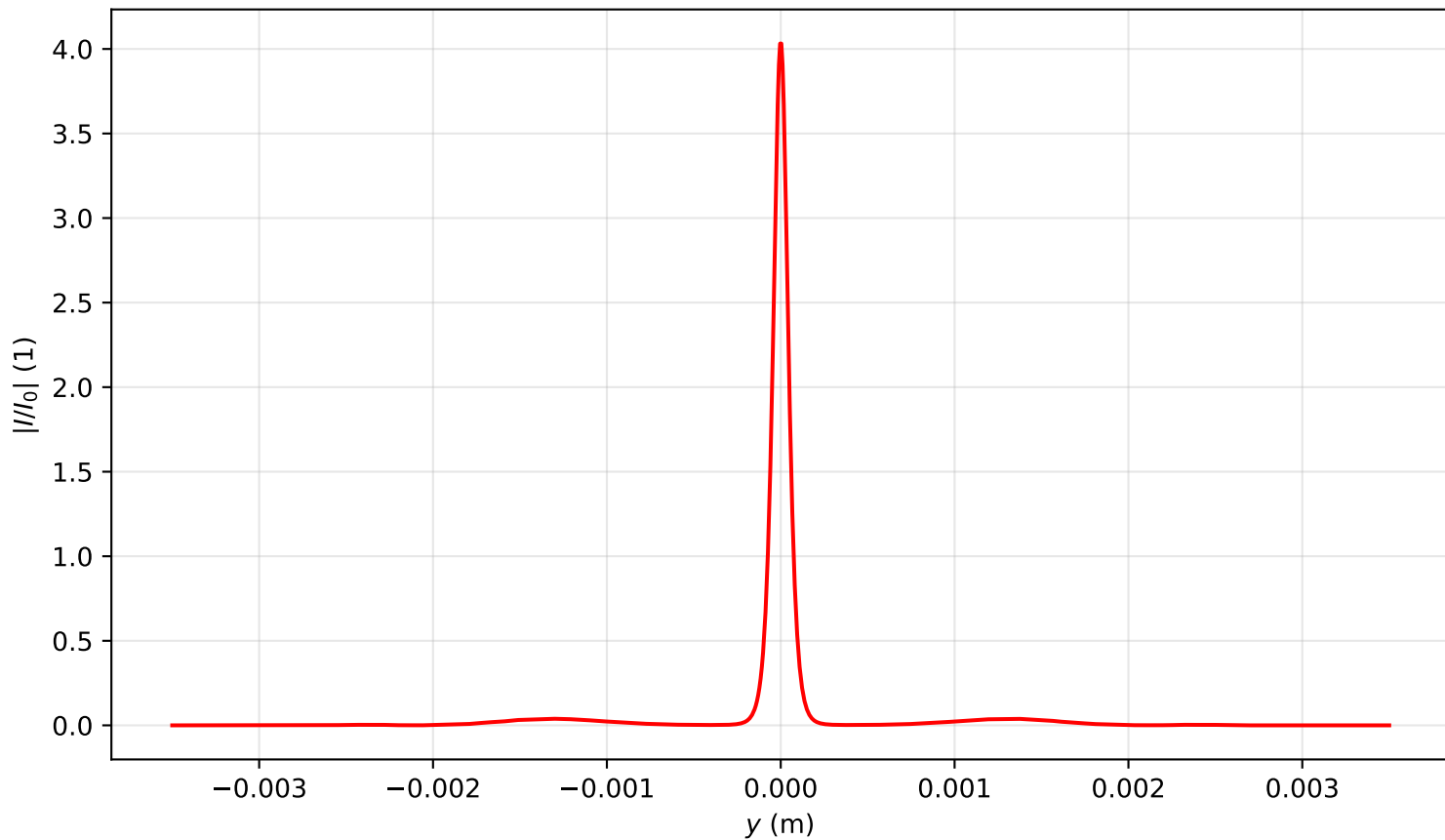
Intensity profile I(x=0, y, z=1.115)/I_0 , P_{in}=8.0P_{cr} , artificial time
